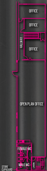
EXISTING FIRST FLOOR PLAN
